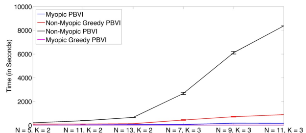
Figure 3: Runtimes for the different methods.
